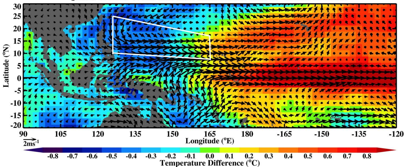
Figure 3. Nature of the physical mechanism behind the TSR primary model in Figure 2. The composite difference figure shows the dominant July-August-September-October (JASO) environmental fields associated with active Northwest Pacific intense typhoon years. Active typhoon seasons occur due to the effects of the anomalous Walker circulation and the resulting weakened easterly trade winds that occur over the tropical Northwest Pacific due to El Niño (warm ENSO) conditions. Inactive typhoon seasons occur due to the effects of the anomalous Walker circulation and the resulting strengthened easterly trade winds that occur over the tropical Northwest Pacific due to La Niña (cold ENSO)
